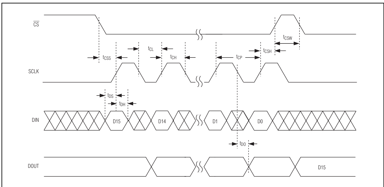
Figure 10. Timing Diagram
